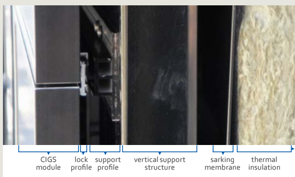
// Cross section of the PV façade system at the ZSW building
