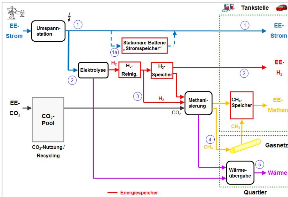
A look at how tomorrow's multi-fuel filling station will work
