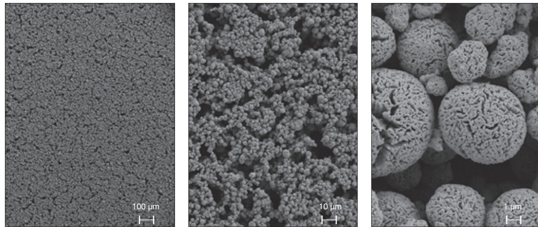
SEM images of surface nickel electrodes showing a coating of nanostructured nickel particles on nickel foil.
