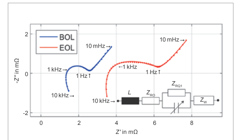
Electrochemical impedance spectra of a cell at the beginning (BoL) and end of life (EoL).
