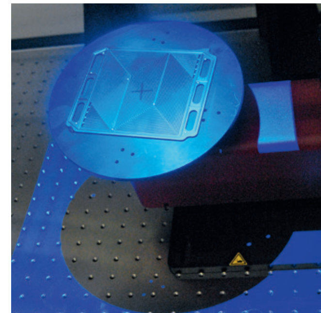
Measuring gas distribution structures using a white light interferometer.
