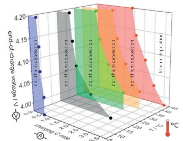
Operating parameters' influence on Li deposition in pouch cells. Source: ZSW/T. Waldmann et al., J. Electrochem. Soc., 163, A1232 (2016).
