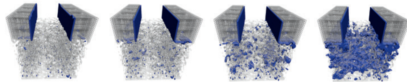
A Monte Carlo simulation showing the effect of varying amounts of PTFE on water distribution in the GDL.
