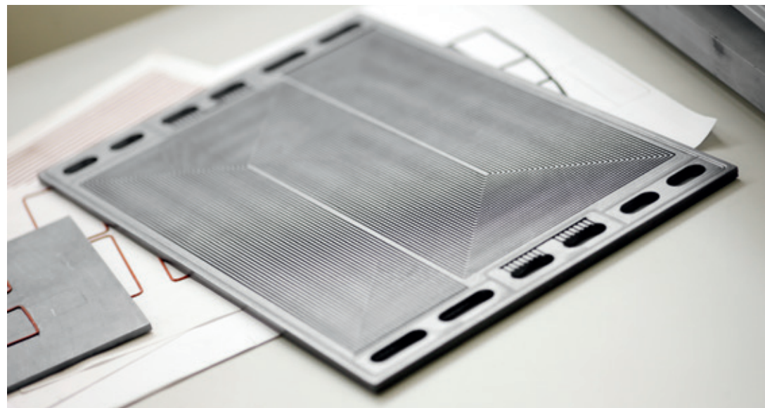
Bipolar plate with an optimised gas manifold structure.
