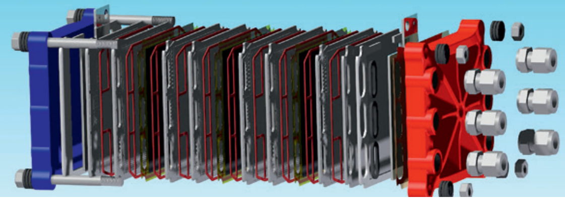
Exploded view of a ZSW fuel cell stack with 100 cm 2 active surface area.
