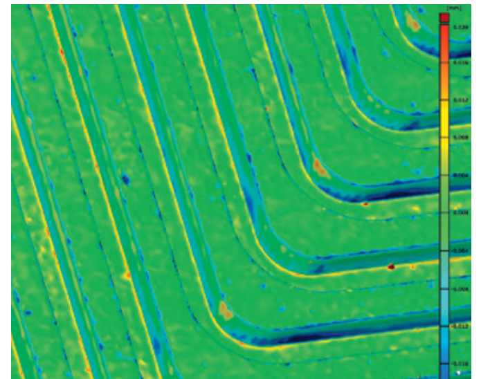
CAD data are compared with measured 3D data to verify bipolar plates' quality.
