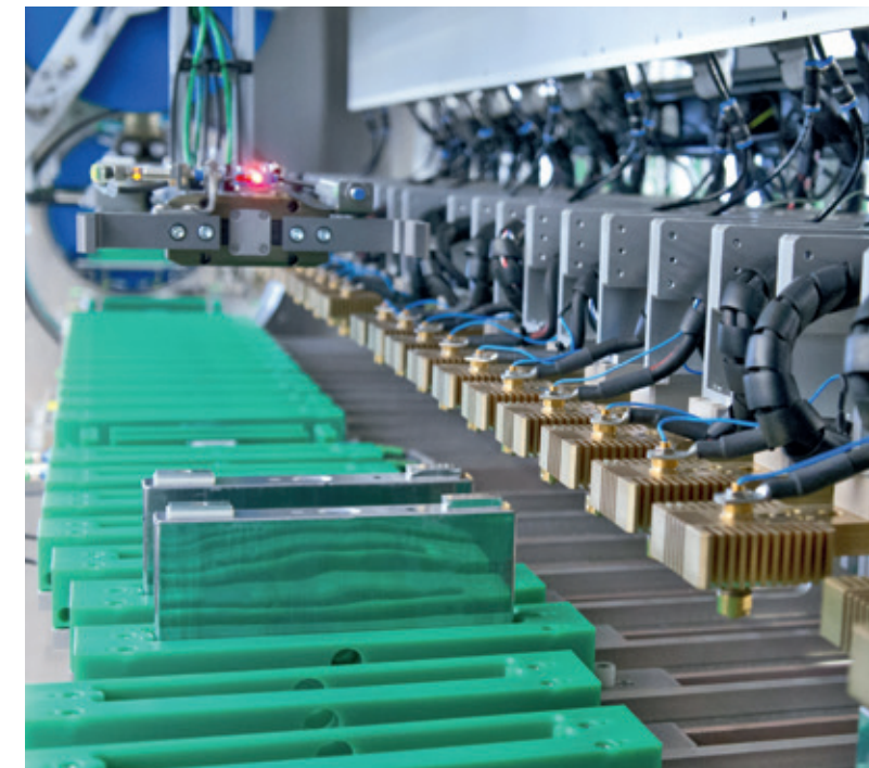
Pre-formation system for wound prismatic cells (PHEV-1 format).
