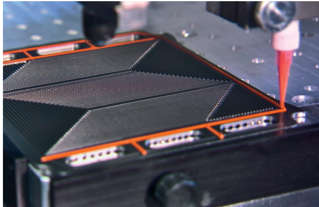
An automated dispenser applies seals.
