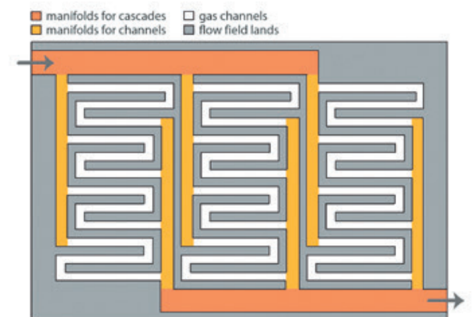
CFD simulation of flow field structures.
