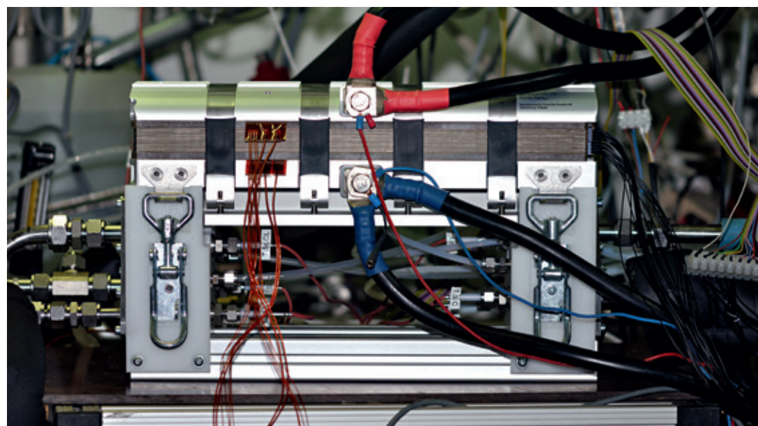
A short stack of a vehicular high-performance fuel cell on the test bench.
