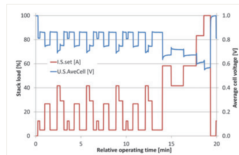
Fuel Cell Dynamic Load Cycle (FC-DLC), a harmonised life-cycle test developed by ZSW.
